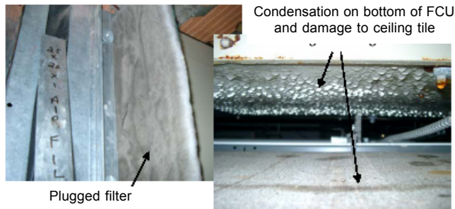
Condensation damage from DX fan coil unit due to plugged filter and low air flow. Large high school.
